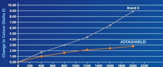
COLOUR RETENTION TEST
